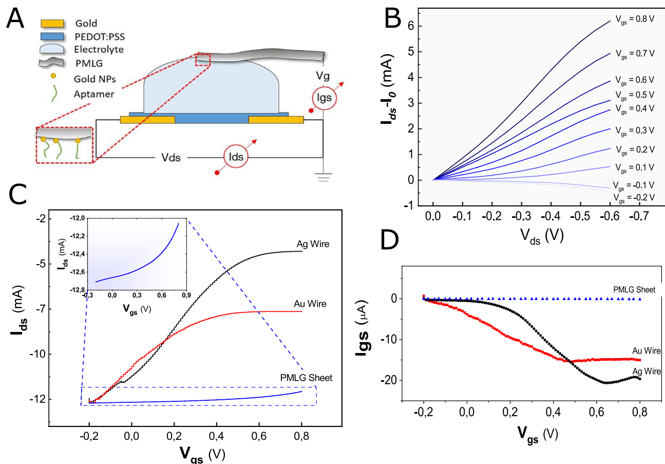
Figure 1. (A) layout of the PMLG gated OECT; (B) related I_{ds}-I_0 versus V_{ds} (from 0 to -0.6 V) recorded using PBS 10 mM as electrolyte (here, I_0 is the current measured at V_{ds} = 0 V) and fixing V_{gs} in the range -0.2 to 0.8 V, step 0.1 V, for each curve; (C) PMLG OECT's transfer characteristics obtained at V_{ds} = -0.25 V for different types of gate electrodes and (D) related gate currents (Ag wire -black line, Au wire—red line and PMLG sheet—blue line). The inset of (C) shows a magnification of PMLG response.
