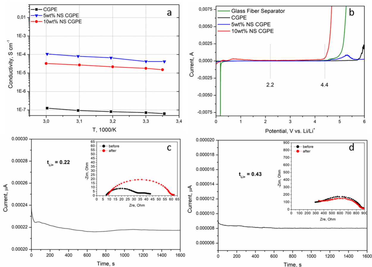
Figure 4. Ionic conductivity vs. temperature plot of the different CGPEs (a), LSV profile of the different CGPEs compared to a commercial glass fiber separator impregnated with liquid electrolyte ( LiTFSI 0.5 M in DMSO) (b). Potentiostatic polarization analysis of a symmetric cell containing the glass fiber separator impregnated with the liquid electrolyte (c) and a symmetric cell containing the CGPE with 5 wt% NS (d).
