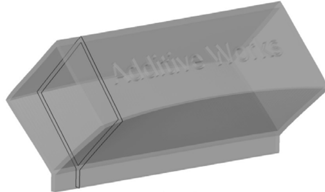
Figure 6. Pre-distorted geometry of the AW Box computed by Amphyon for compensation of the SLM distortions.
