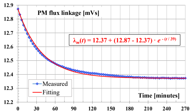
Fig. 13. Decay of the PM flux linkage for MUT_3 .
