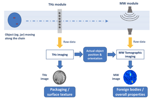
Fig. 1: Conceptual scheme of the EM technology for food monitoring.
