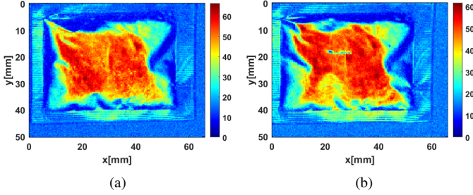
Fig. 7: False color THz image (a) Standard packaging; (b) Defect packaging.
