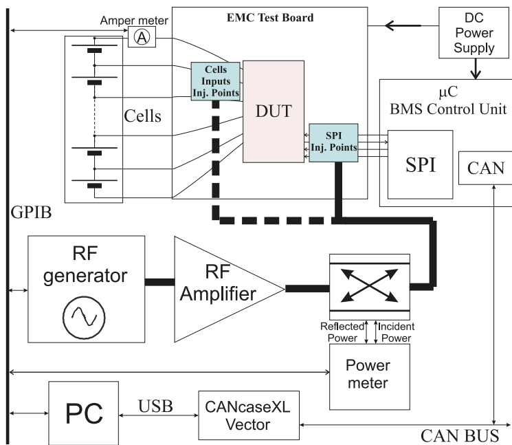
Figure 3. Direct power injection. Experimental test setup.
