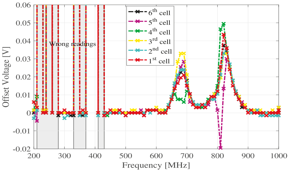
Figure 13. EMI-induced offset in the cell voltage readings. Antenna in front of the EUT (Figure 12). Vertical polarization.
