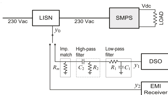
Figure 1. Scheme of the experimental setup: SMPS under test and its dc variable load, LISN (Line Impedance Stabilization Network), 50 \Omega impedance matching, high-pass filter (1 kHz cutoff) and low-pass filter (2 MHz cutoff), Digital Storage Oscilloscope (DSO) and EMI Receiver.
