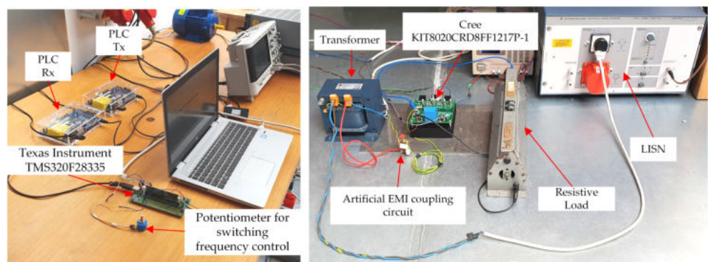
Figure 4. Setup testbed.
