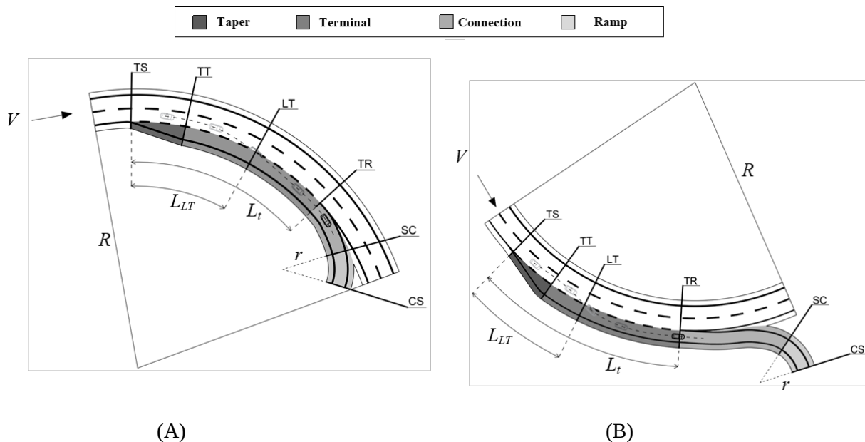
Figure 1 Geometric factors considered in the design of continue (A) and reverse (B) terminals include motorway radius ( R ), terminal length ( L_t ), and traffic volume ( V ). Ramp radius was assumed constant in the experiment ( r = 150 m). Significant termini: terminal start (TS), taper-to-terminal (TT), lane-to-terminal (LT), terminal-to-ramp (TR), spiral to curve (SC), curve to spiral (CS).
