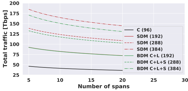
Fig. 7. Total allocated traffic vs. number of fiber spans for all upgrade scenarios.
