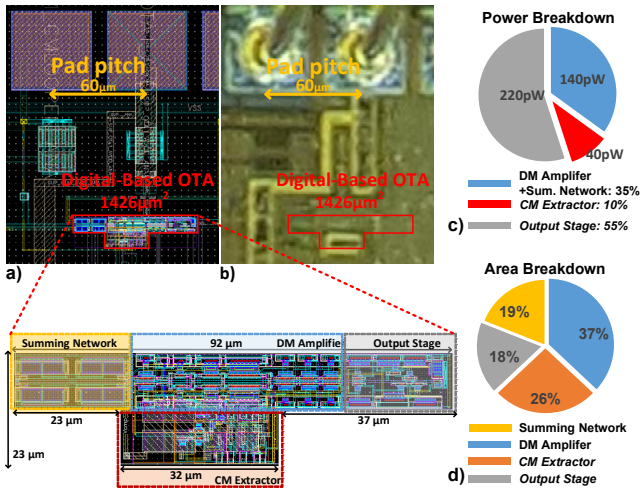
Fig. 4. a) Layout view of the DB-OTA, b) micrograph of the 180-nm test-chip, c) power breakdown, and d) area breakdown.
