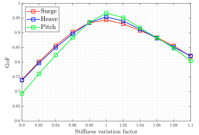
Fig. 7. Stiffness matrix influence on the estimation
