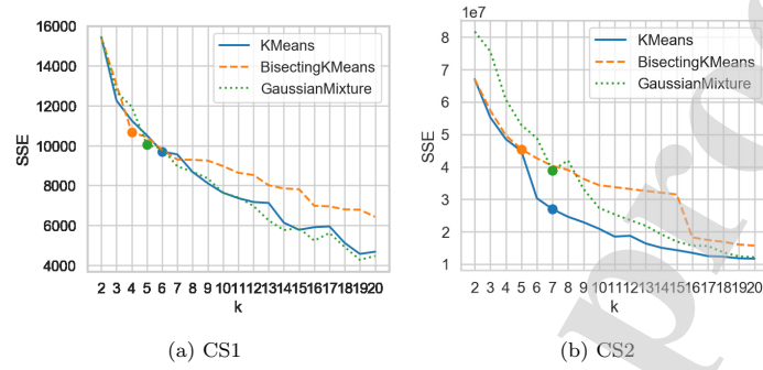
Figure 7: Elbow method, SSE trends against k for all clustering algorithms, selected values of k are indicated by a filled circle.
