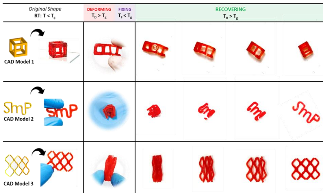
Figure S3. Shape memory cycles of different DLP – printed structures from PHEMA-co-PEGMEMMA 65:35. Temporary shape programmed by deforming the structures above the T_g ( T_D = 70^\circ\text{C} ) and fixing the strained configuration by rapid cooling below the T_g ( T_F = 3^\circ\text{C} ). The shape recovery is carried out in water heated to above the T_g ( T_R = T_D = 70^\circ\text{C} ).
