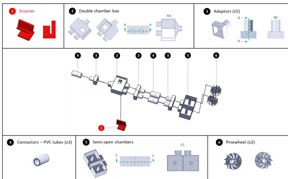
Figure S4. CAD models of the device components with assembly instructions.
