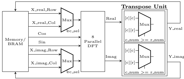
Fig. 3 RTL diagram of DFT2 unit
