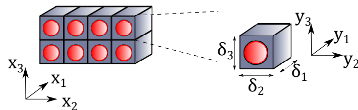
Figure 4. Representation of a periodic heterogeneous material and its RUC along with the global and local coordinate reference frames.
