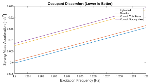
Figure 9. Representative sample of Occupant Discomfort of four tested cases below 1.4 Hz
