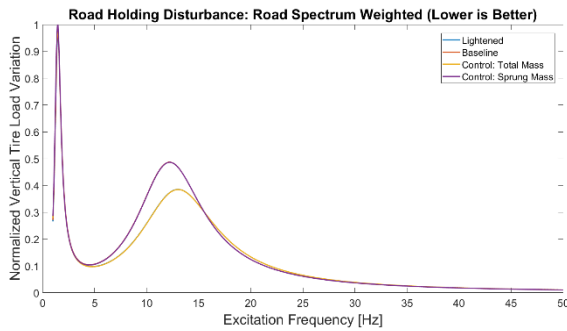
Figure 14. Road Spectrum Weighted Road Holding Disturbance
