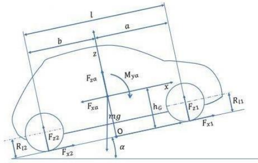
Figure 19. Free body diagram
