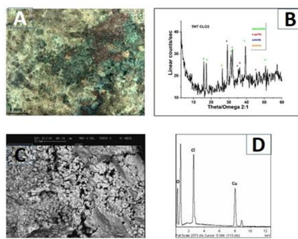
Figure 5. Coin THT CLO3: OM image (A), XRD spectrum (B), SEM image (C) and EDS spectrum (D).
