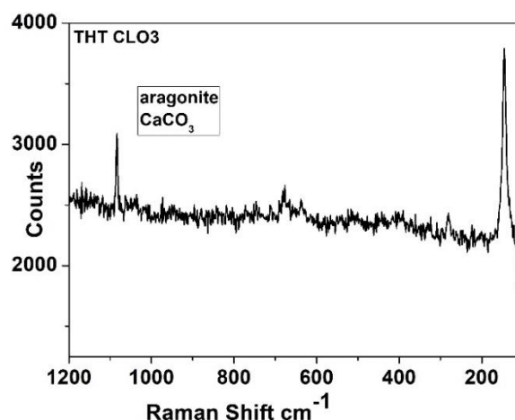
Figure 9. Raman spectrum of aragonite ( \text{CaCO}_3 ) on coin THT CLO3.
