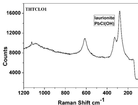
Figure 8. Raman spectrum of laurionite [PbCl(OH)] on coin THT CLO1.
