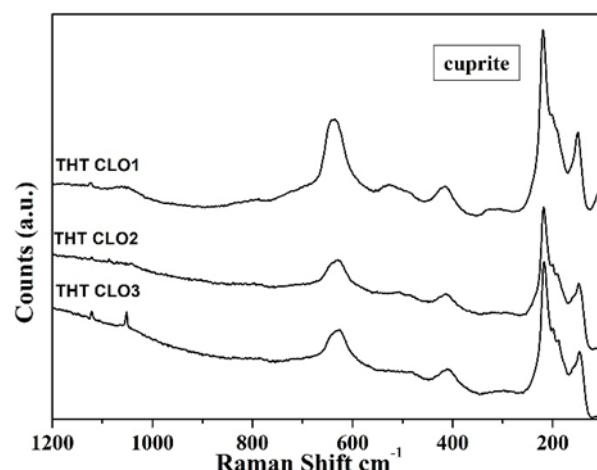
Figure 7. Raman spectra of cuprite ( \text{Cu}_2\text{O} ) on the coins found at Tharros. The Raman spectra collected in a Cu-rich area evidence the presence of poorly crystallised cuprite.
