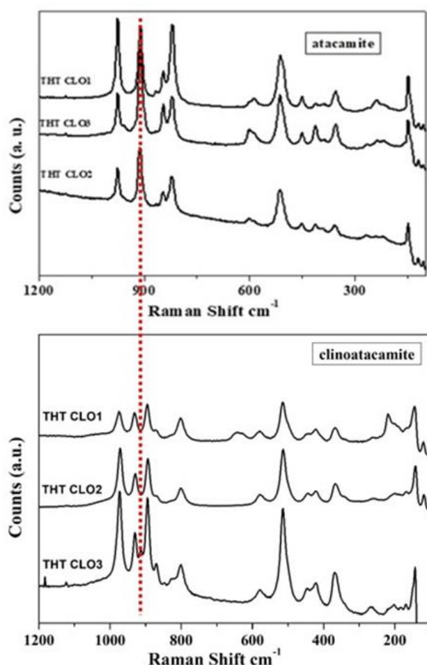
Figure 6. Raman spectra of copper trihydroxychlorides [\text{Cu}_2\text{Cl}(\text{OH})_3] atacamite and clinoatacamite on the coins found at Tharros.
