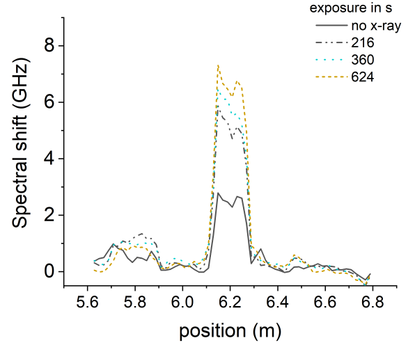
Fig. 10. Spectral shift versus position along the fiber for different times of exposure at 2 Gy/min.
