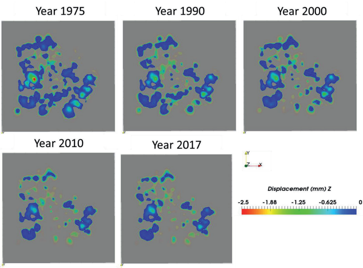
Fig. 5 - Maps of the simulated vertical displacement (in mm) relevant to the average compressibility values of Table 2 for years 1975, 1990, 2000, 2010, and 2017.
