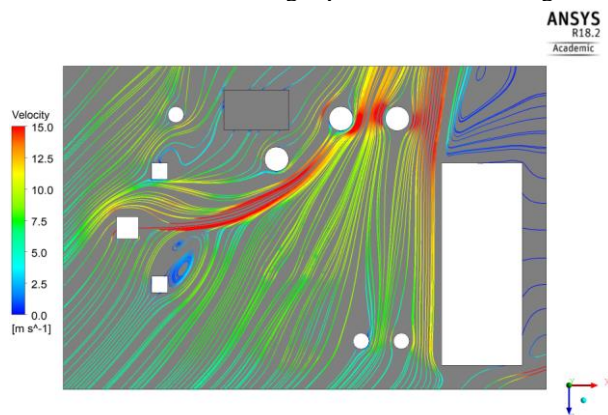
Figure 6: Velocity field in the production deck
