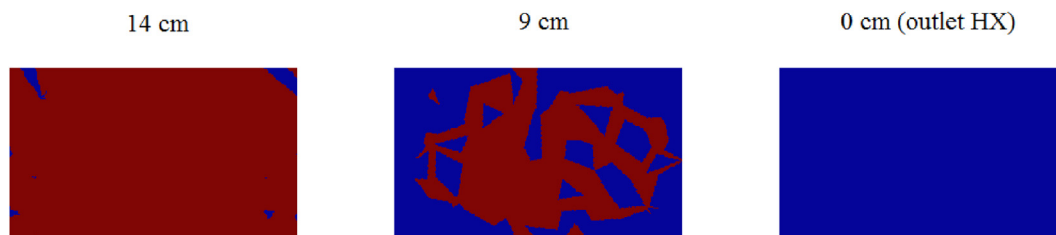
Fig. 14. Multi-physics PCE results: Multiple cross sections of the heat exchanger, at different heights (measured from the outlet), showing the region in which T_F > 923 K with a probability higher (red) or lower (blue) than 95%. As energy is progressively transferred to the secondary loop, the salt cools down increasing the probability to have a temperature below the threshold.
