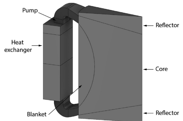
Fig. 3. MSFR geometry used simulations, showing the main regions considered in the model. Only one recirculation loop was modeled, given the symmetry of the problem. From Tiberge et al. (2020b).
