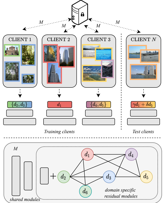
Figure 1. In a federated scenario, clients and server exchange the parameters of the model M . Each client has access to its local data, which can be non-i.i.d. and unbalanced. In the image, each color identifies a different distribution, i.e. a domain, such as pictures of skyscrapers or sea landscapes. Our model M is made of domain-agnostic layers (in gray) and a GCN containing domain-specific parameters, added as residual. According to the domains of the input images, the corresponding nodes of the GCN are activated. At test time, new domains can be addressed as a soft combination of the discovered ones, e.g. skyscrapers over the sea.
