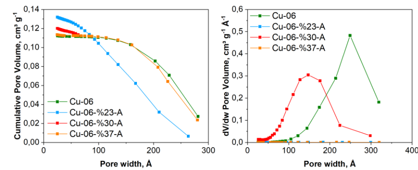
Figure 4. Pore size distribution.
