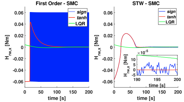
Fig. 4. Comparison of the torque around X_{body} with LQR and SMC. ( f = 5\text{ Hz} )
