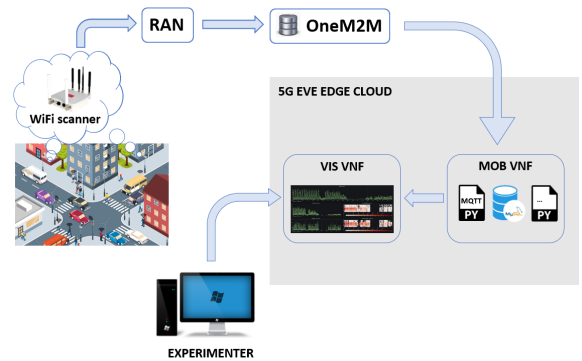
Fig. 1: 5G EVE Edge Cloud testbed architecture by which the data collected by the WiFi scanner is processed through two VNFs [3]
