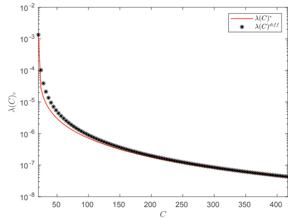
Fig. 3. Optimal variance of the arithmetic mean \lambda(C)_v^* compared with \lambda(C)_v^{\text{diff}} .
