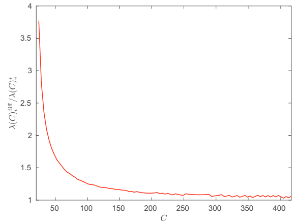
Fig. 4. Ratio between \lambda(C)_v^* and \lambda(C)_v^{\text{diff}} as function of C .
