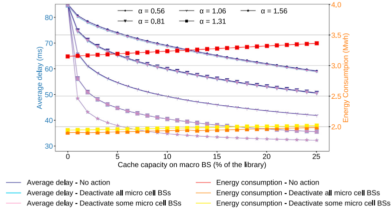
Fig. 6. Delay and energy consumption varying the size of each cache, for different values of the parameter \alpha , when No action and Deactivate all micro cell BSs are used.
