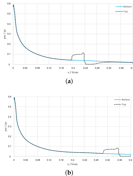
Figure 6. Wall pressure distribution on LP40 with \dot{m}_i/m_T = 0.1 with injection slot at x/L = 0.6 (a) and x/L = 0.9 (b).
