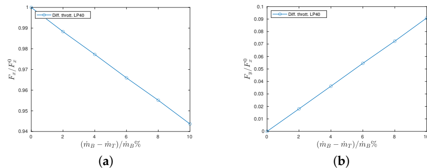
Figure 8. Axial (a) and lateral (b) thrust components obtained by differential throttling on LP40 geometry.
