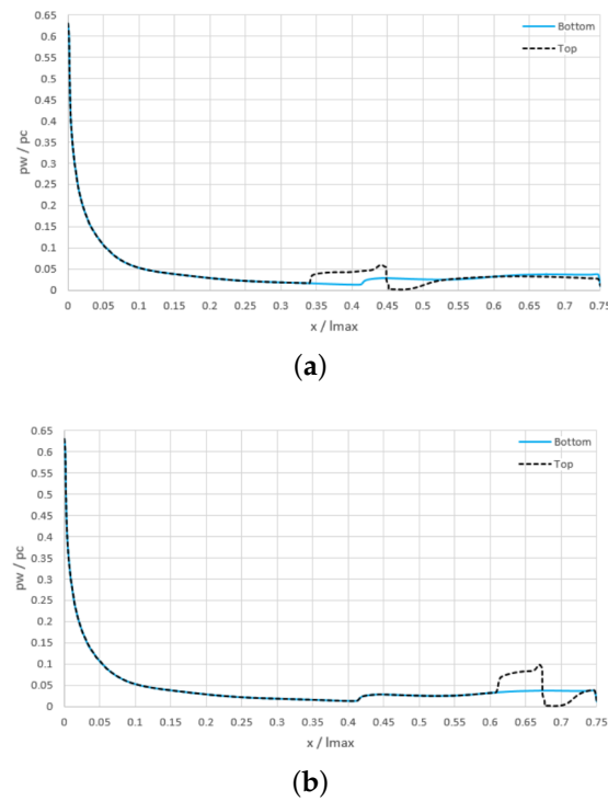
Figure 10. Wall pressure distribution on LP75 with \dot{m}_i / \dot{m}_T = 0.1 with injection slot at x/L = 0.6 (a) and x/L = 0.9 (b).
