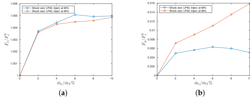
Figure 7. Axial (a) and lateral (b) thrust components obtained by shock vector control on LP40 geometry.
