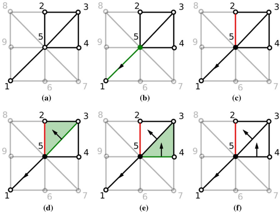
Fig. 3 Working example for the subroutine HomotopyExpansion . Each image in the figure represents an operation performed at a specific line with respect to the code in Appendix A: a the input lower star of vertex 5; b Vertex 5 is paired to edge [1,5] at line 8; c Edge [2,5] is found critical at line 24; d edge [3,5] is paired to triangle [2,3,5] at line 17; e edge [4,5] is paired to triangle [3,4,5] at line 17; f the discrete gradient vector field retrieved by HomotopyExpansion
