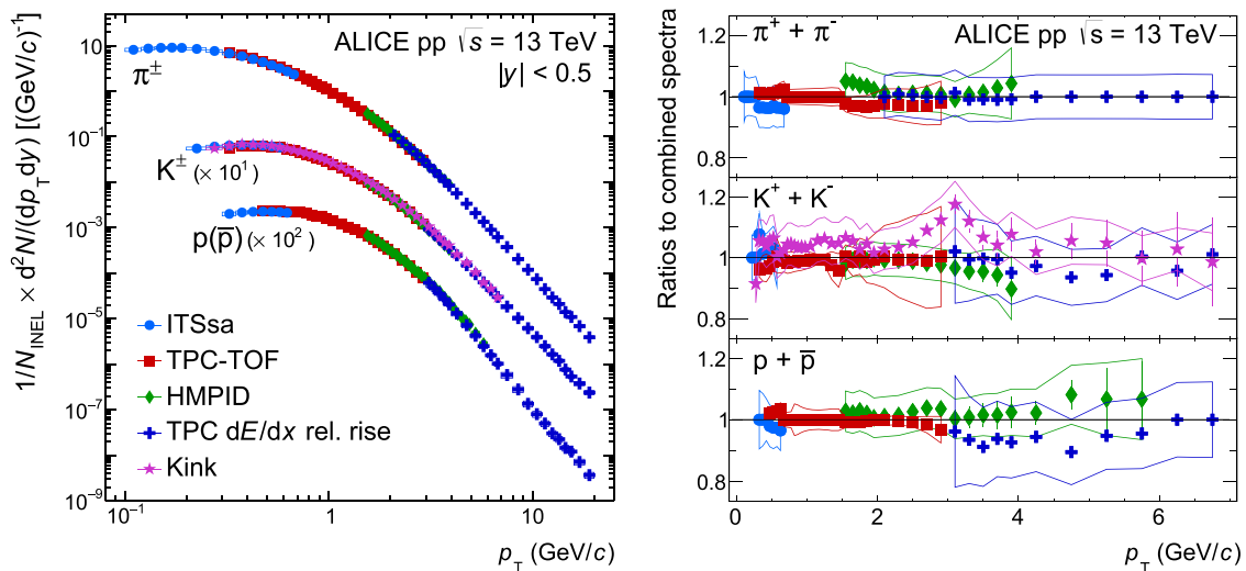
Fig. 3 Left panel: p_T spectra of \pi^\pm , K^\pm , and p(\bar{p}) measured at midrapidity ( |y| < 0.5 ) in pp collisions at \sqrt{s} = 13 \text{ TeV} using different PID techniques. The spectra are normalized to the number of inelastic collisions. Right panel: The ratios of individual spectra to the com-
