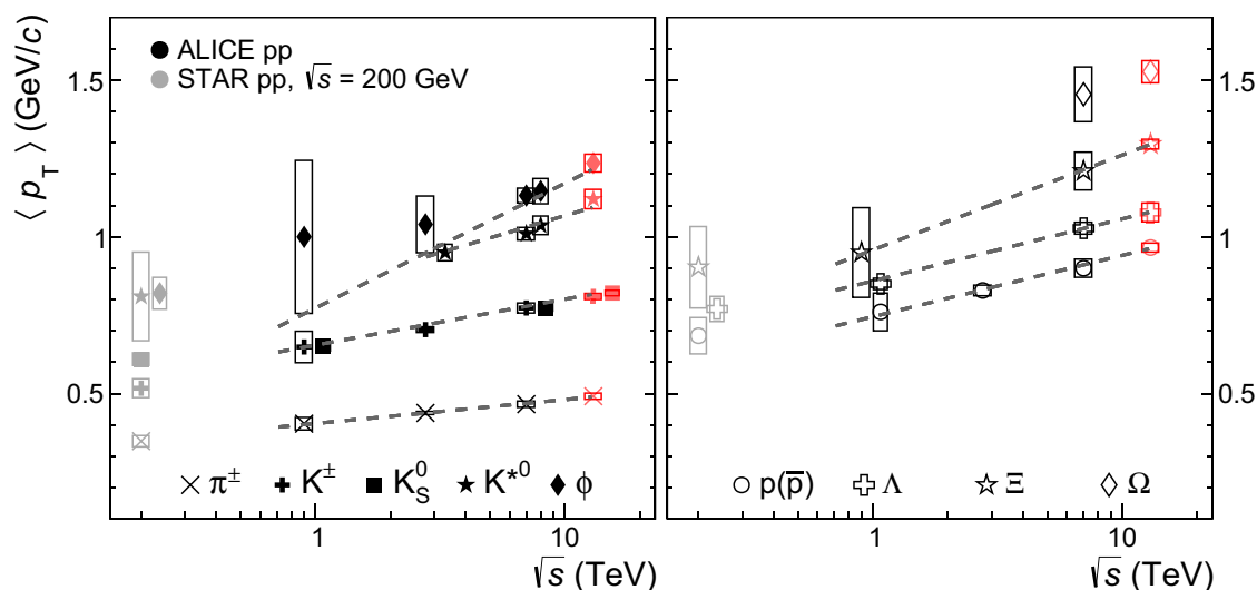
Fig. 10 Average transverse momentum \langle p_T \rangle as a function of the center-of-mass energy. Open boxes indicate the statistical and systematic uncertainties (when available) summed in quadrature. Results from ALICE [7,24,26,27,51,58,60,63] are compared with those from STAR measured at \sqrt{s} = 200 GeV [88]. Some data points are slightly offset
