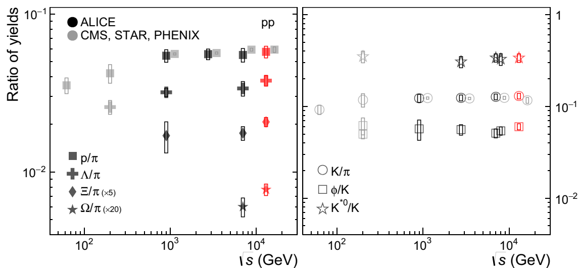
Fig. 11 Ratio of particle yields to \pi^\pm and K^\pm as a function of the collision energy \sqrt{s} (GeV). Results from ALICE [7,24,26,27,51,58,60,63] are compared with those from CMS [90] at the same energies, and with those from STAR [88,91,92] at \sqrt{s} = 200 GeV and PHENIX [19,20]
