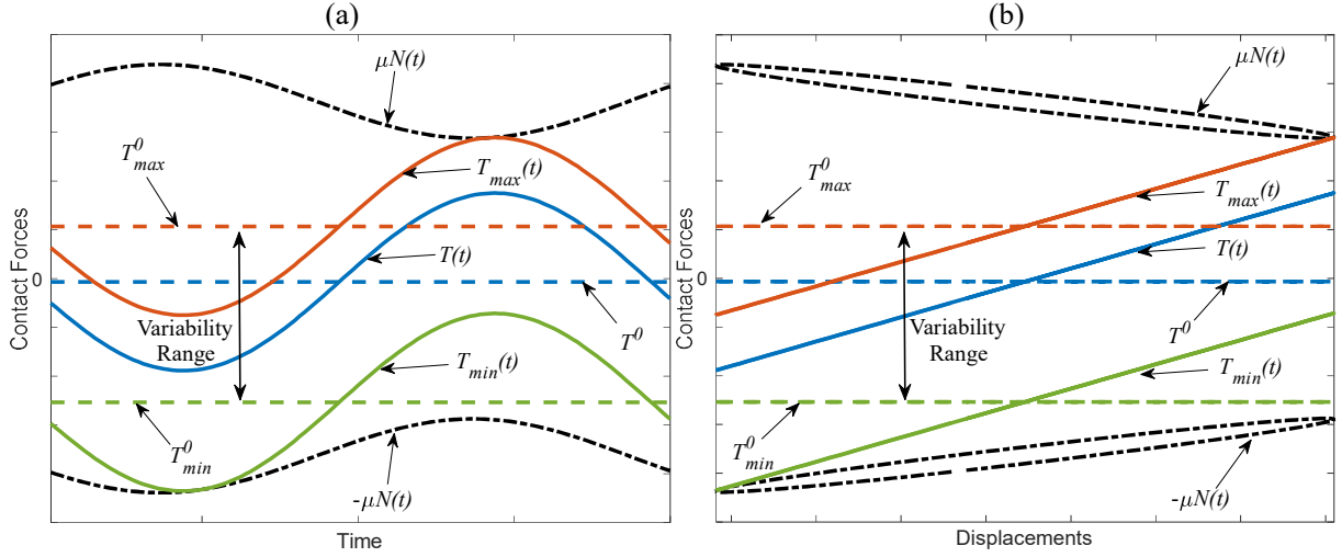
Fig. 3 (a) Time Histories of Contact Forces, (b) Hysteresis Curves for a Full Stick Cycle [25]
