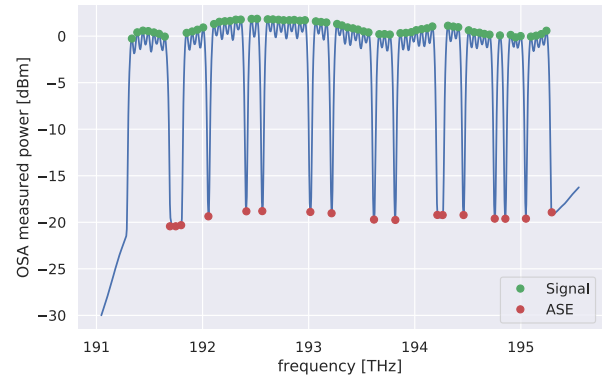
FIGURE 5. The power measured using the end-of-line OSA for one of the 2520 spectral load configurations. Channels which are turned on provide signal power measurements, whereas channels which are turned off provide ASE noise power measurements.
