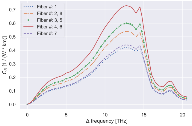
FIGURE 6. Final SRS efficiency curves deduced and used for each fiber span.
