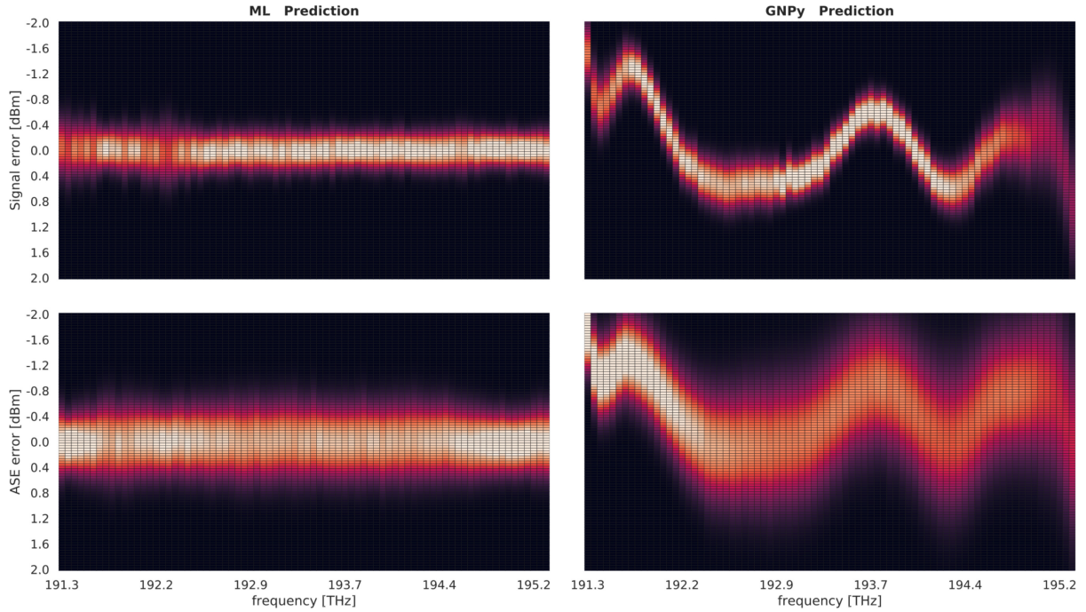
FIGURE 9. Error distribution of the signal and ASE noise prediction obtained with the the ML models and the GNPpy engine, respectively.
