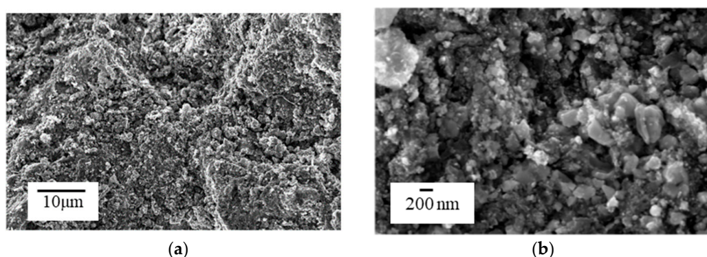
Figure 7. FESEM image of the biochar filler: (a) overview at magnification of 10 m; (b) magnification of 200 nm showing the granular aspect of biochar.
