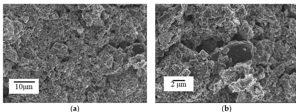
Figure 8. FESEM images of biochar films: (a) overview of biochar film at magnification of 10 m; (b) magnified at 2 m, biochar film still retains granular aspect.
