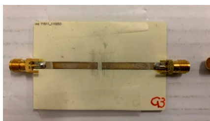
Figure 1. Prototype of the microstrip line with gap without film deposition.
