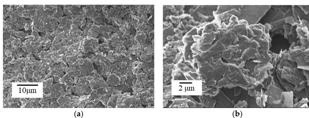
Figure 9. FESEM images of graphene films: (a) overview of graphene film at magnification of 10 m; (b) magnified at 2 m, flakes embedded in graphene film can be seen.
