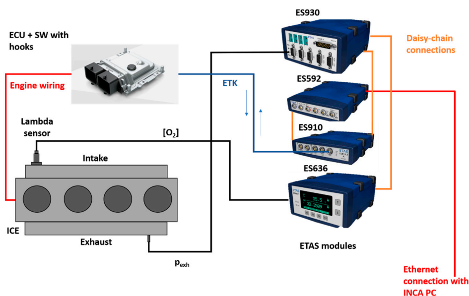
Figure 8. Daisy-chain configuration for the different ETAS modules.
