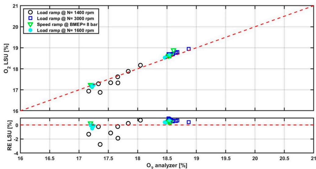
Figure 10. Intake O_2 concentration: measurements of the lambda sensor unit (LSU) analyzer vs. test cell analyzer for the different ramp tests.
