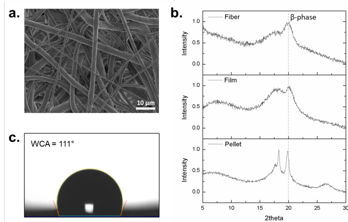
Fig. 1: a. PVDF-HFP electrospun membrane, b. XRD spectra of PVDF-HFP, c. water contact angle of a PVDF-HFP fibrous membrane.
