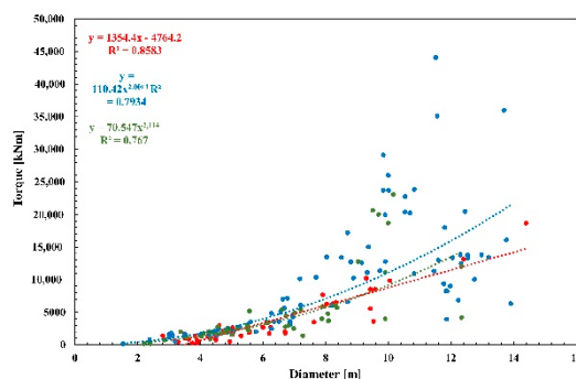
Figure 2. Correlation between diameter and torque. Red: open TBM; blue: single shield TBM; green: double shield TBM.
