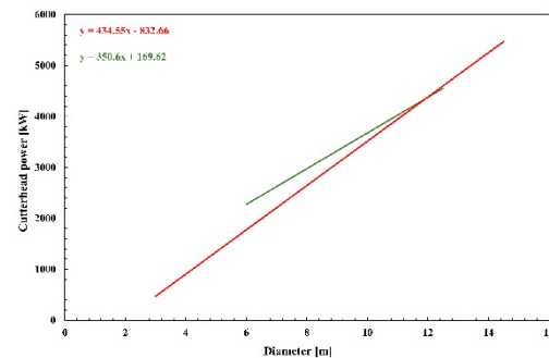
Figure 20. Trend of the power vs. the diameter based on data collected from the analysis of open TBMs. In red, the experimental model proposed in this study; in green, the model proposed by [43].
