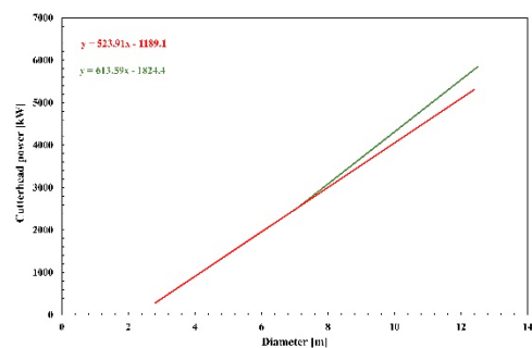
Figure 25. Trend of the power vs. the diameter based on data collected from the analysis of double shield TBMs. In red, the experimental model proposed in this study; in green, the model proposed by [43].
