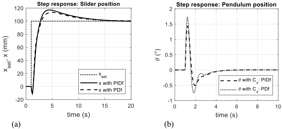
Fig. 6. Step response with two different compensators C_x , (a) slider position and (b) pendulum position.
