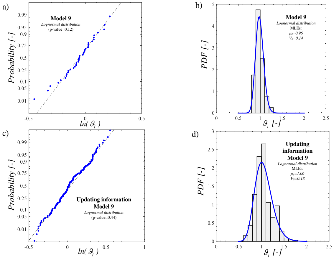
Fig.5. Probability plot of \ln(\mathcal{Q}_i) for the Model 9 (a) and its updating information (c); Relative frequency histogram and lognormal PDF of the ratio \mathcal{Q}_i for the Model 9 (b) and its updating information (d).
