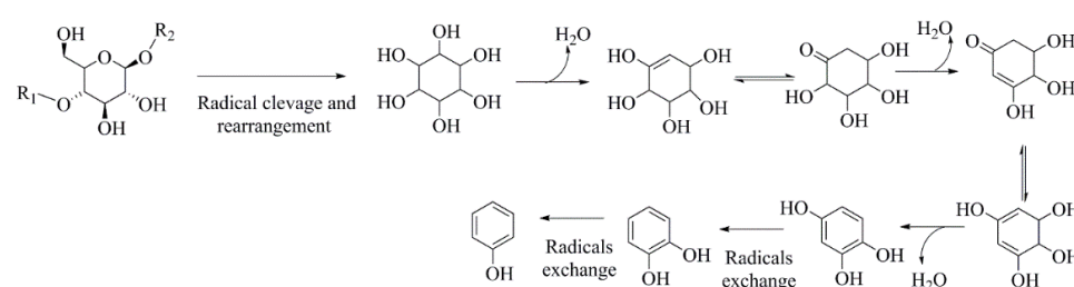
Figure 2. Chemical pathway of aromatics formation during MAP of cellulose as reported by Bartoli et al. [26].
