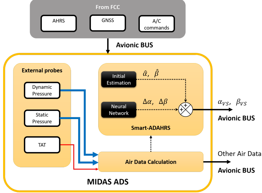
Figure 1: High-level schematic of the MIDAS ADS.
