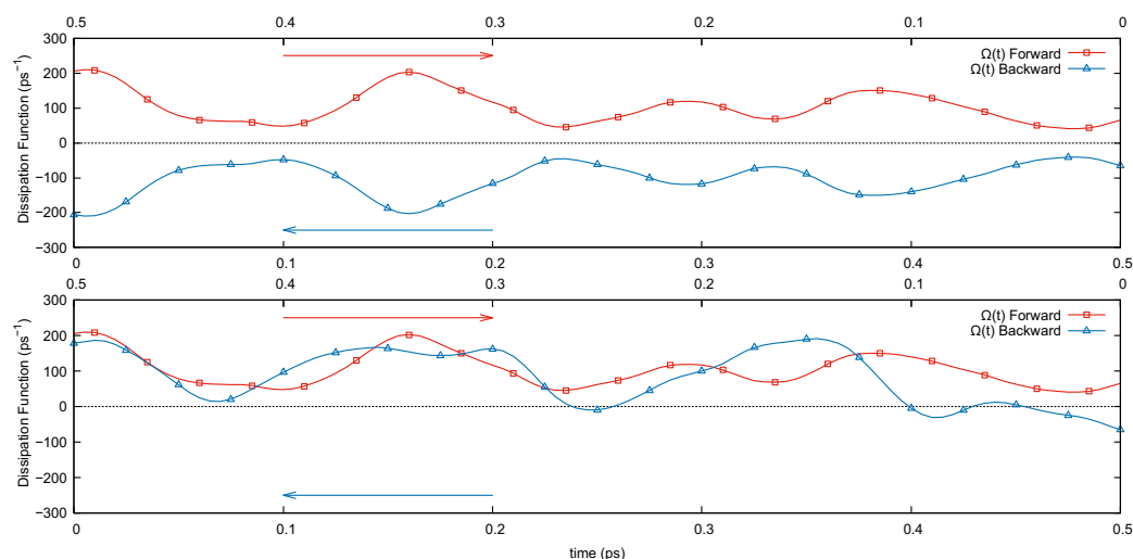
Figure 1. Instantaneous dissipation function from Equation (8) for 500 fs of the “forward” evolution (red curve, open squares) and for 500 fs of the “backward” trajectory (blue curve, open triangles) obtained via \mathcal{M}_{\text{ext}}^{(3)} (upper panel). The opposite values of the dissipation demonstrate the odd signature under the generalized time-reversal transformation used. The same behavior is not observed when the backward trajectory is obtained applying \mathcal{M}_s^{\text{ext}} (bottom panel) as the presence of the magnetic field breaks the symmetry of the system under this transformation. Results are for the nonequilibrium simulation set-up described in Section 3 for liquid NaCl.
