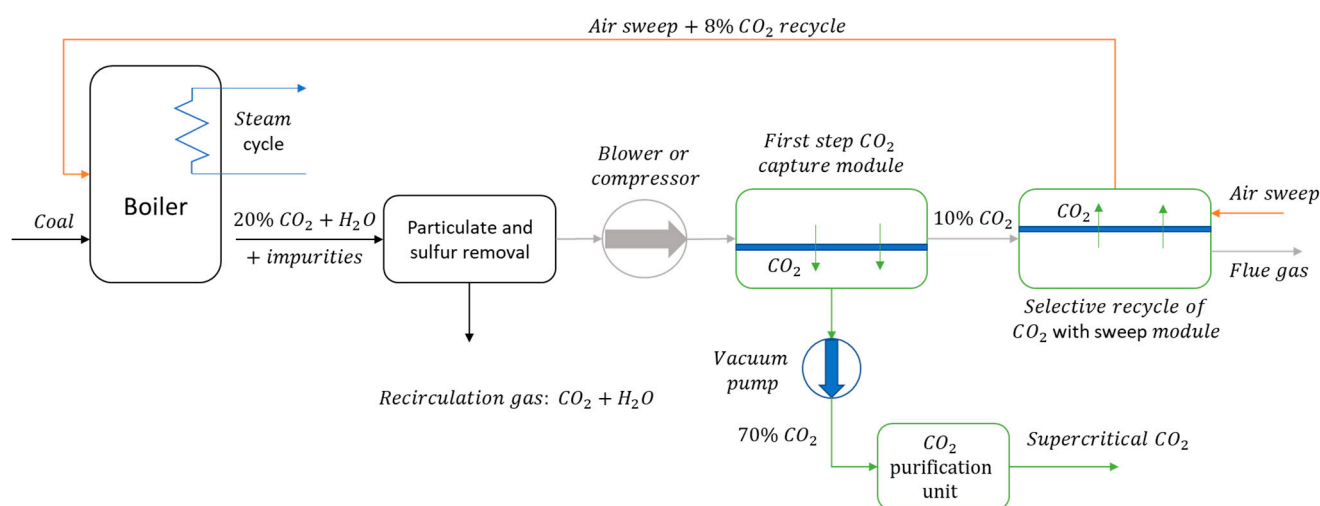
Figure 8. Simplified diagram of the Membrane and Technology Research Institute (MTR) selective recycle \text{CO}_2 capture process at a coal-fired power plant using Polaris™ membrane in separation modules [22].
