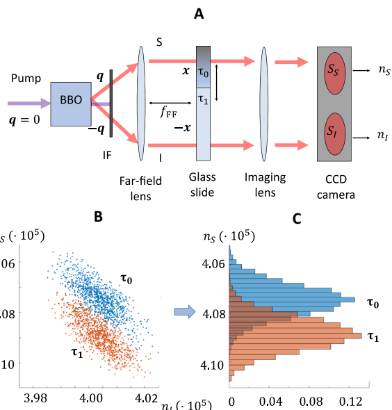
Fig. 3. Simplified schematic of the experimental setup and photon number distributions. (A) In the \beta -barium borate (BBO) crystal, the multimode TMSV source is generated. The signal beam passes through the memory cell investigated, whose transmissivity can be either \tau_0 or \tau_1 and is then detected in the S_S region of the charge-coupled device (CCD) camera. The idler beam goes directly to the S_I region of the CCD. n_S and n_I are the total photon counts over S_S and S_I . IF, interferential filter ( 800 \pm 20 ) nm. (B) n_S in function of n_I , for 1000 frames. Blue dots correspond to \tau_0 \sim 0.996 , while red dots correspond to \tau_1 = 1 . (C) n_S relative frequency distribution for \tau_0 \sim 0.996 (blue histogram) and \tau_1 = 1 (red histogram).
