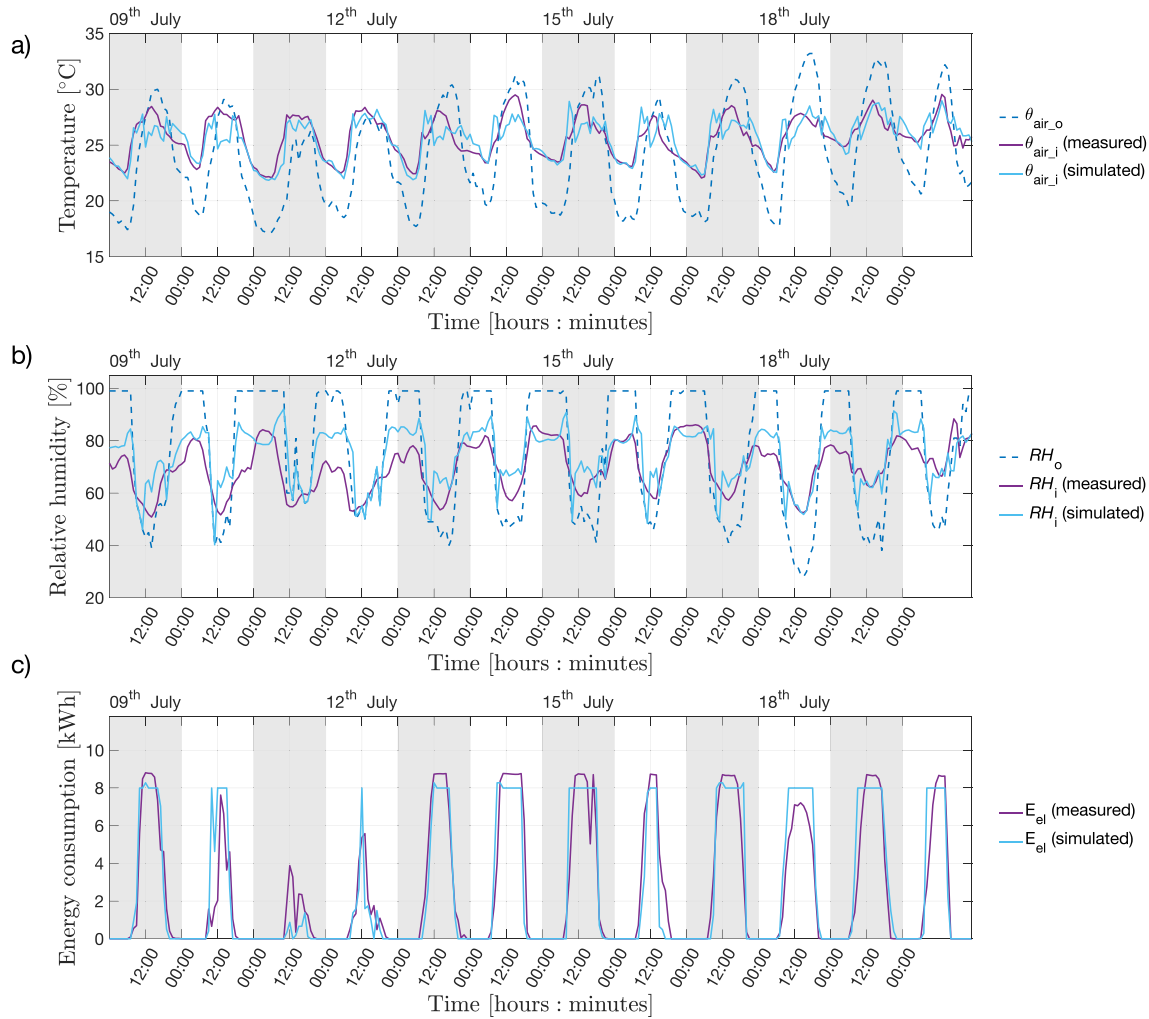
Fig. 14. Trends of monitored and simulated values of (a) indoor air temperature ( \theta_{\text{air-i}} ), (b) relative humidity ( RH_i ), (c) and hourly electrical energy consumption. The outdoor air temperature ( \theta_{\text{air-o}} ) and relative humidity ( RH_o ) are also showed.
