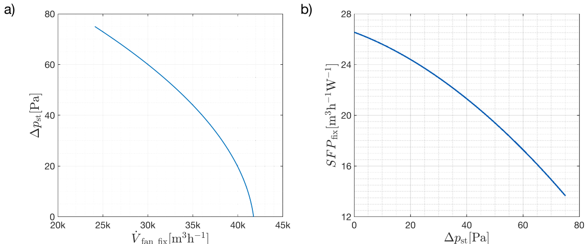
Fig. 7. Fixed speed fan (a) flowrate and (b) Specific Fan Performance ( SFP ) as function of fan static pressure.
