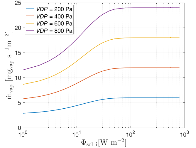
Fig. 3. Evapotranspiration rates ( \dot{m}_{vap} ) calculated as a function of the solar radiation on the canopies ( \phi_{sol,i} ) and the water Vapour Pressure Deficit ( VPD ) according to Eq. (5) (x-axis is in logarithmic scale).
