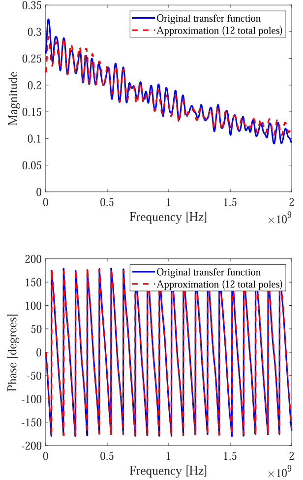
FIGURE 6. Magnitude and phase plots of the reconstructed transfer function of example 2.
