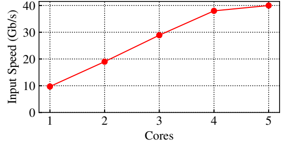
Fig. 6: Performance with four input and four output interfaces using the ISP-FULL trace.
