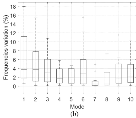
Figure 2. Boxplots of the absolute values of the variation of the natural frequencies: (a) for all modes accordingly to the damage scenario and (b) for all damage scenarios according to the mode number. The central line indicates the median value, the bottom and top edges of the box indicate the 25-th and 75-th percentiles, and the whiskers the largest and smallest data points not considered outliers. The plus symbol indicates the outlier values.
