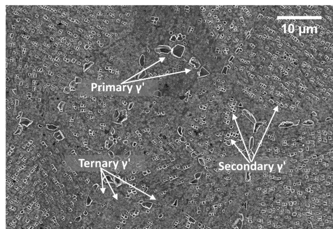
Figure 2. Generic micrograph showing the three \gamma' categories, i.e., primary, secondary and ternary.
